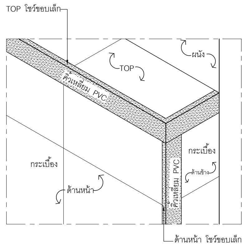
DETAIL (D5) TOP LOWWALL
